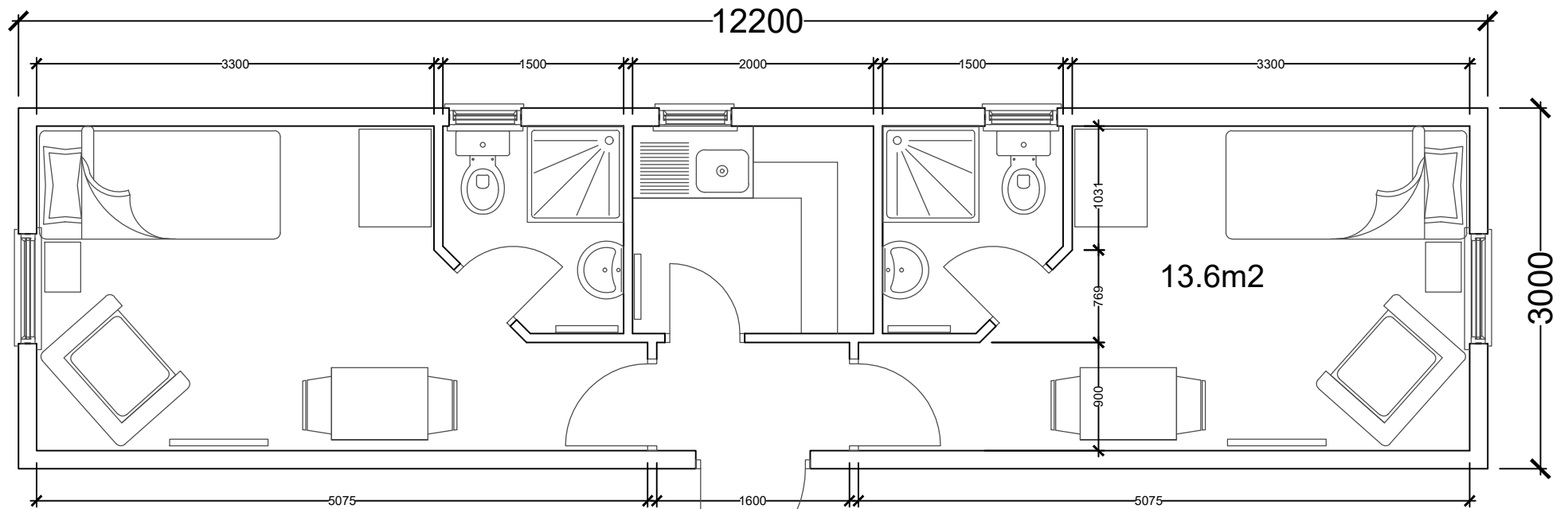
POD FLOOR PLAN - Shared Kitchen (1:50)
