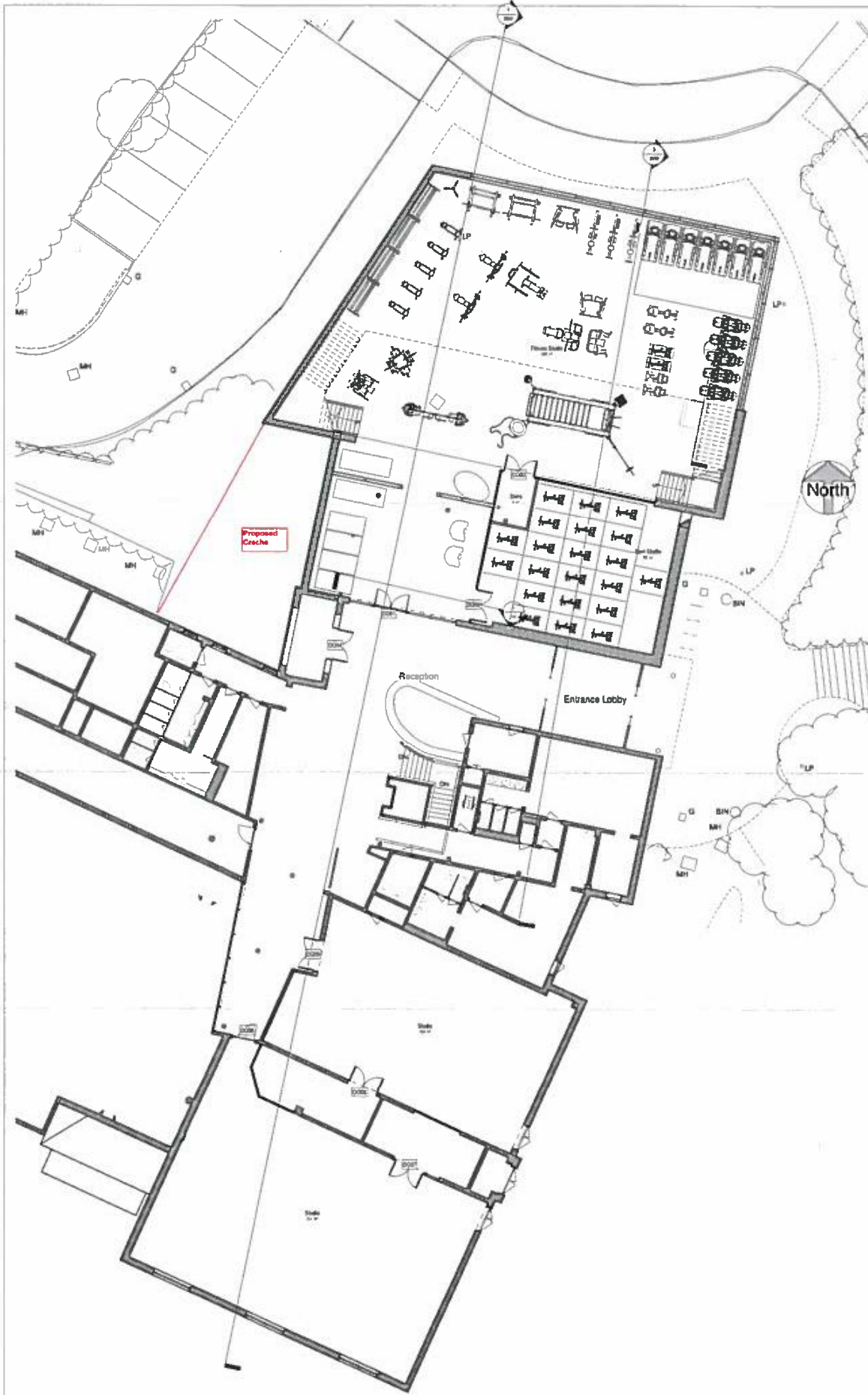
1 Proposed Ground Floor Plan 1/100
